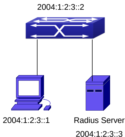
Figure 6-17 IPv6 Radius
