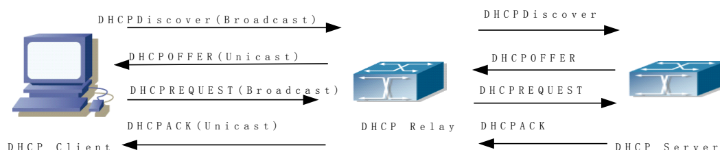
Figure 3-10 DHCP relay
