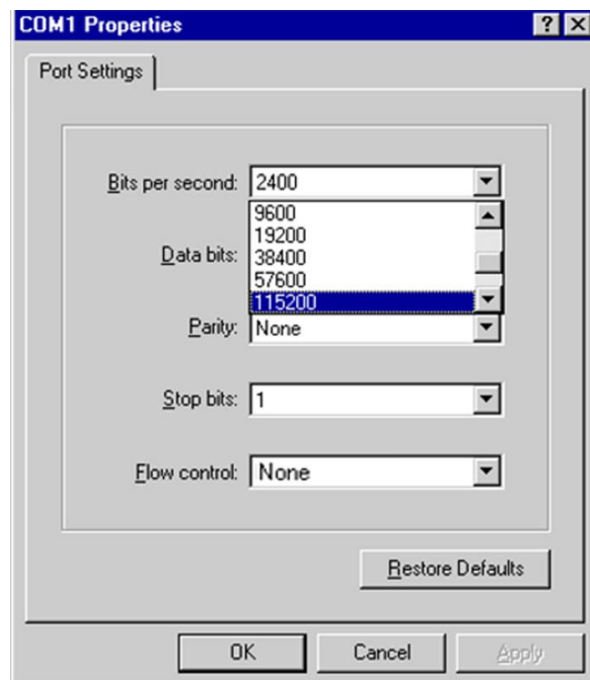
Figure 1-5 Opening HyperTerminal
