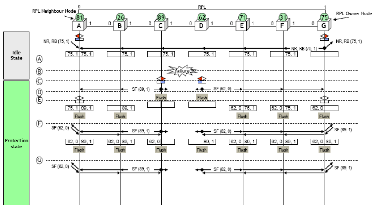
Figure 7-15 single-link fault
